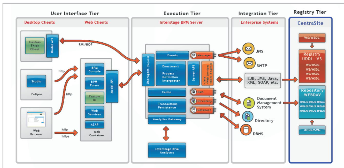
Figure 21 – Interstage BPM SOA Architecture
