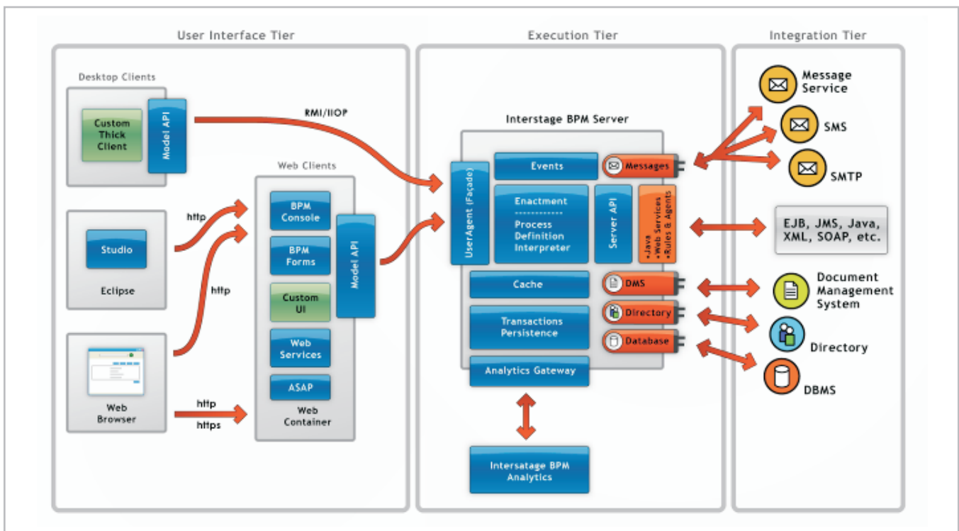
Figure 11: Interstage BPM Architecture
